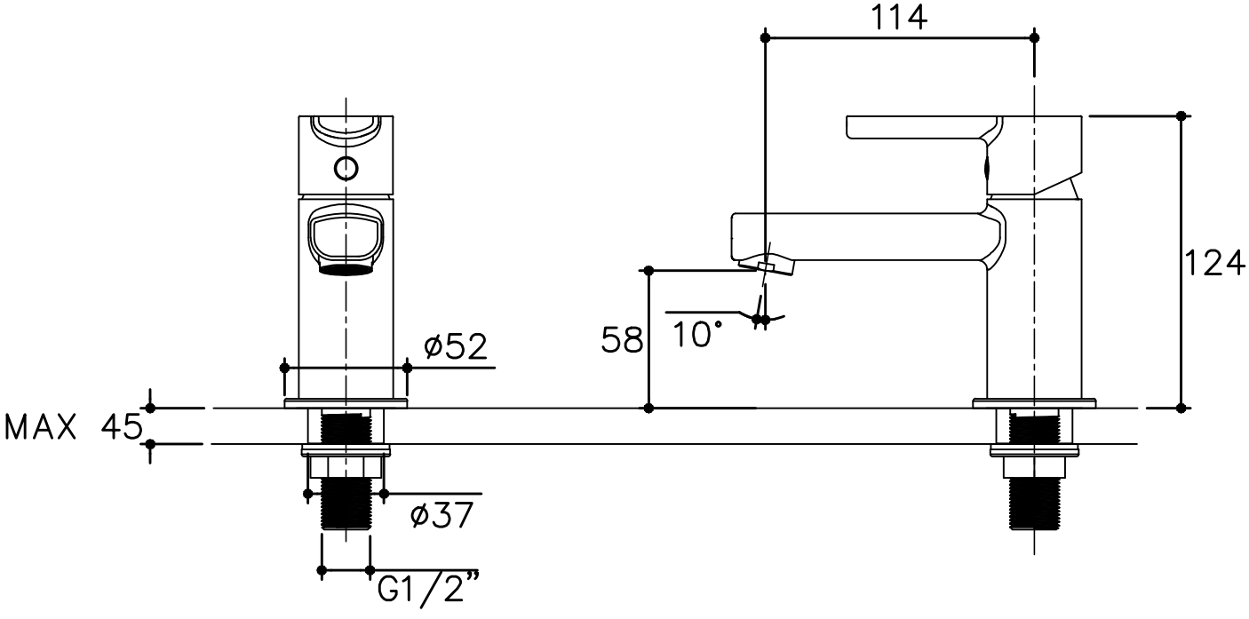
Product Diagram 98096X-4-CP
