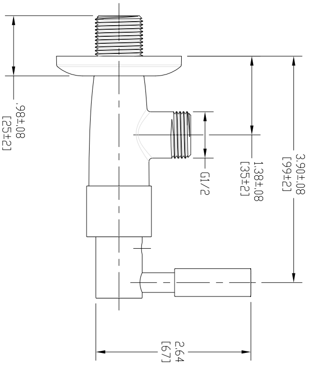
PATD SHOWER VALVE, CW
