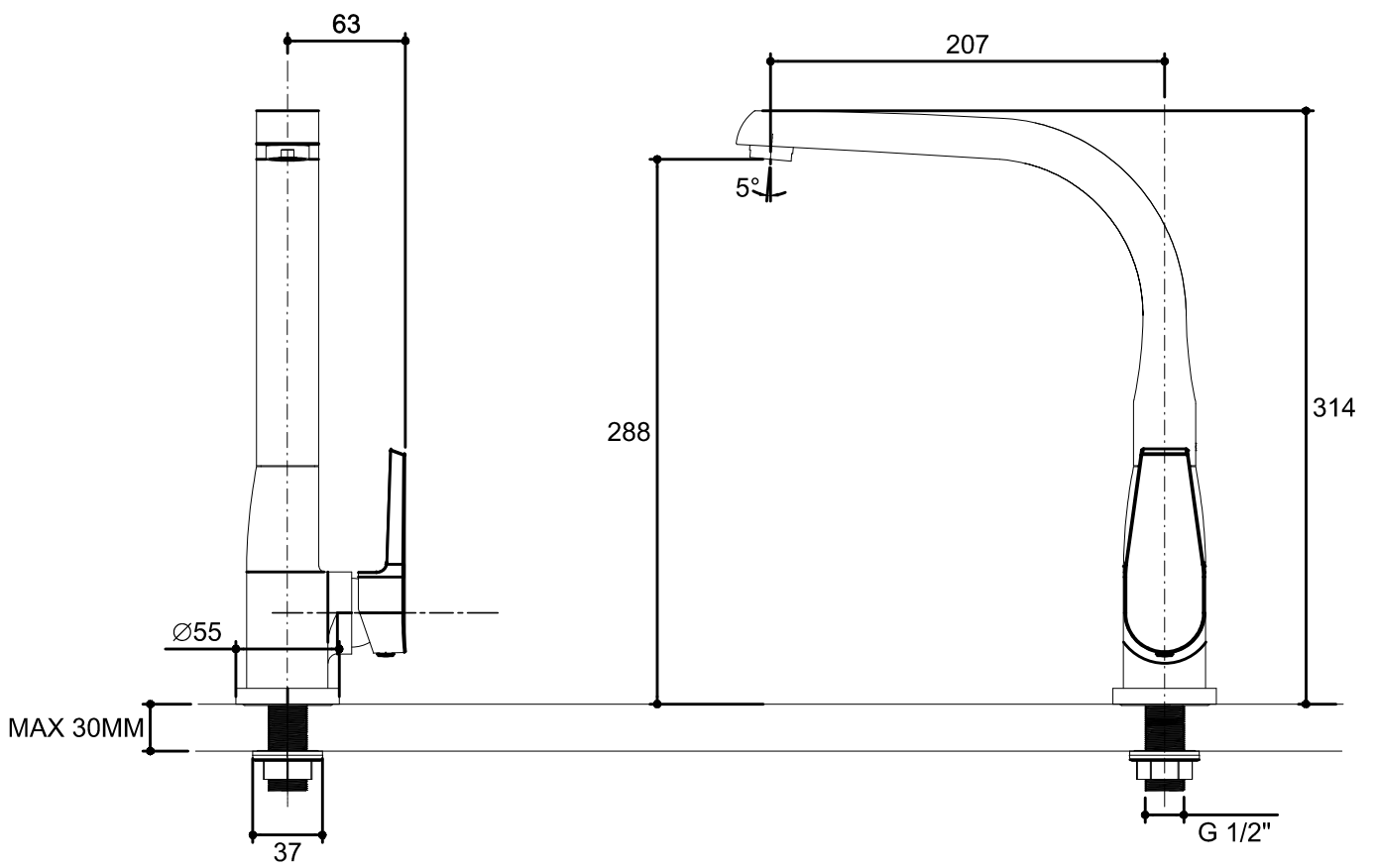
Product Diagram P7706X-4-CP
