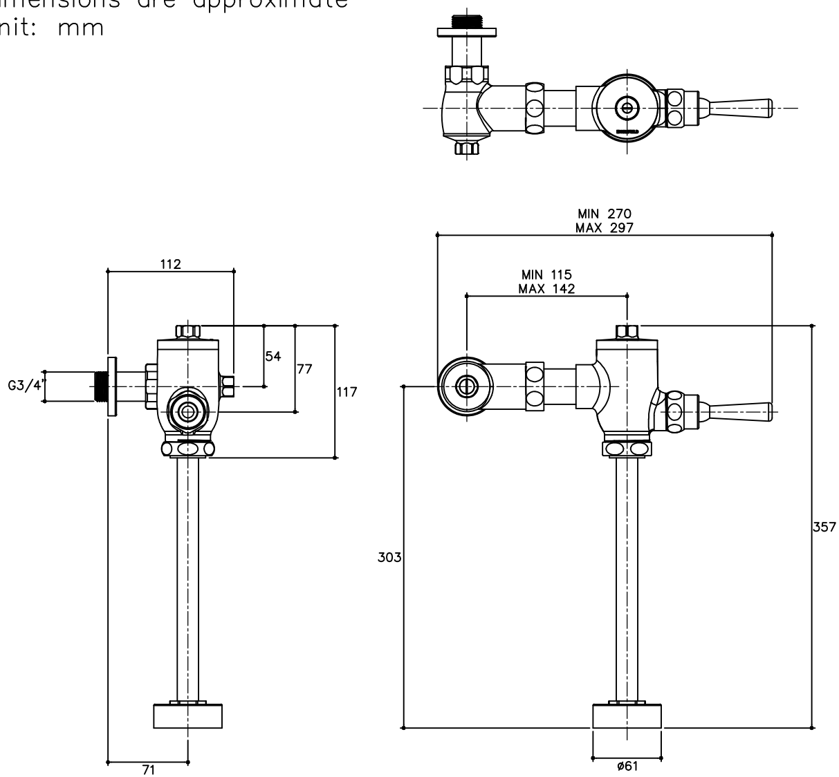
Product Diagram 98095X-CP
