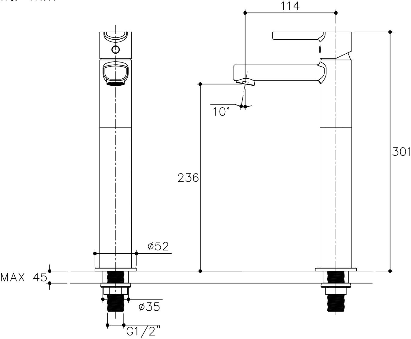
Product Diagram 98097X-4-CP
